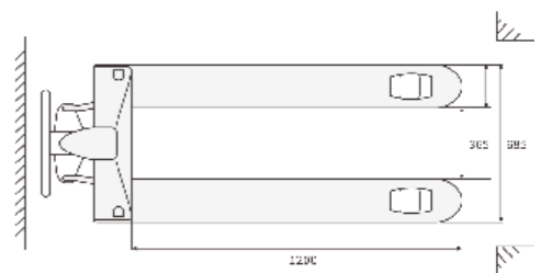
Model 685 pallet jack
