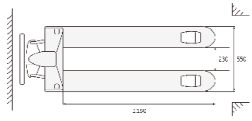
Model 550 pallet jack
